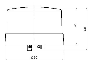
Ø80mm
