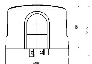
Ø80mm(window)
